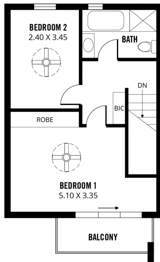
UPPER LEVEL
