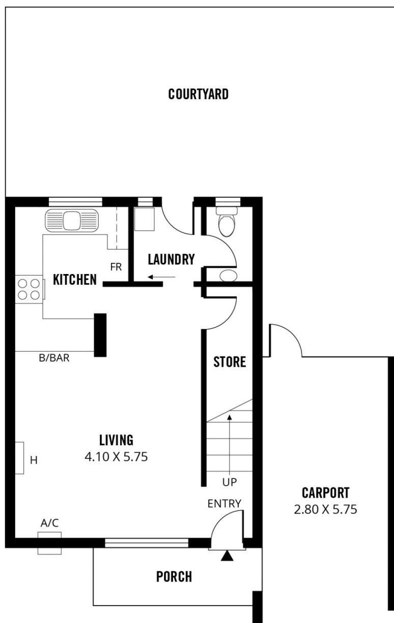
LOWER LEVEL
